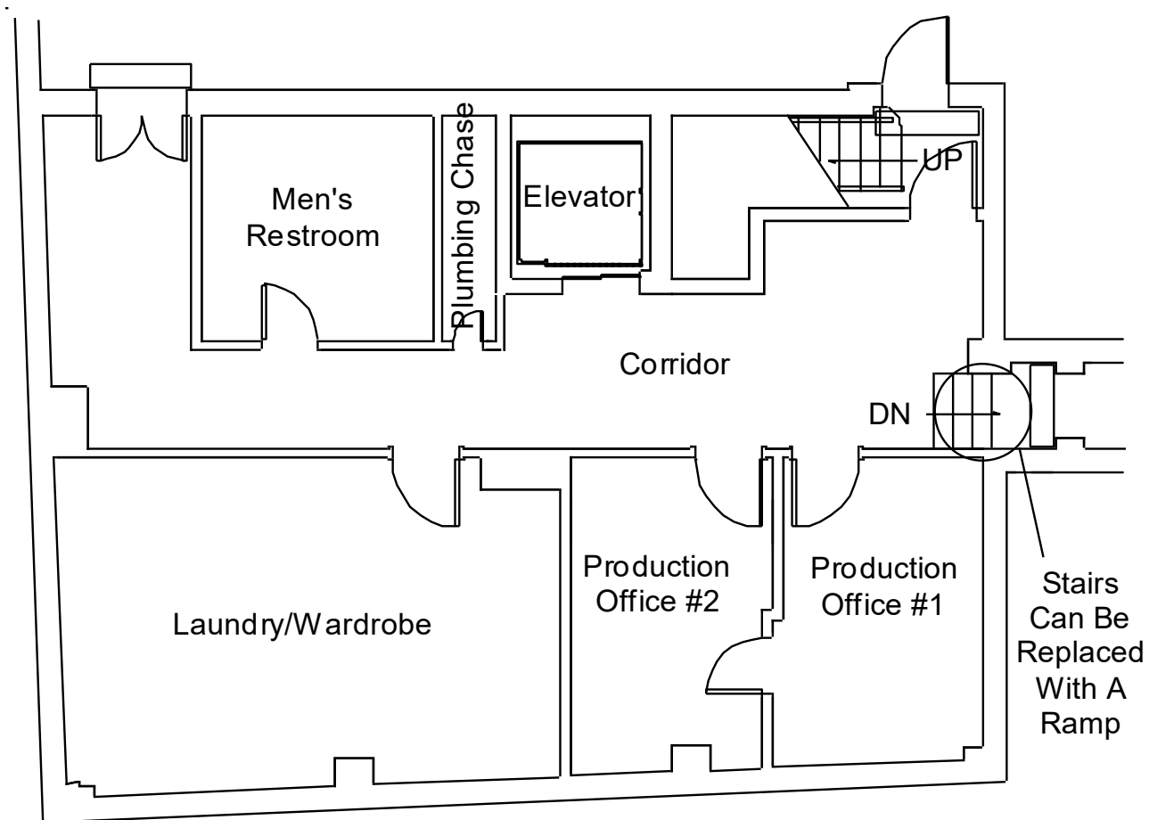
Basement Plan
